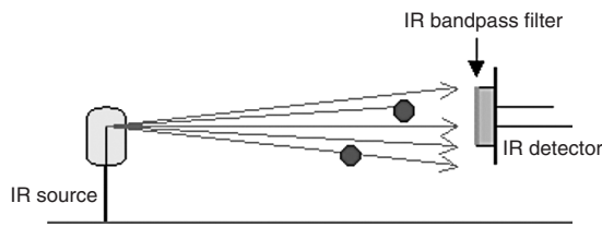
Figure 11. Simplified diagram of a single beam IR absorption gas detector.
